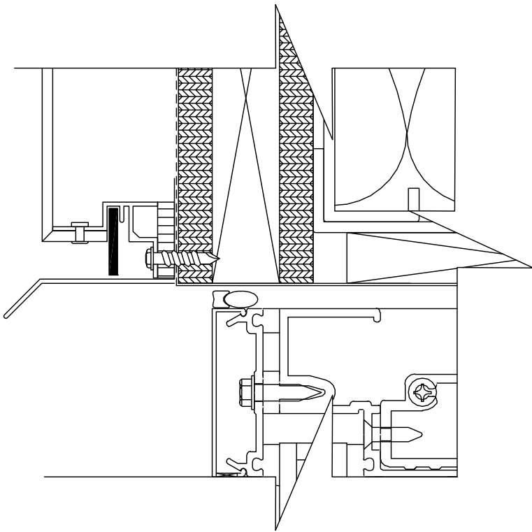
WINDOW / DOOR HEAD S40
