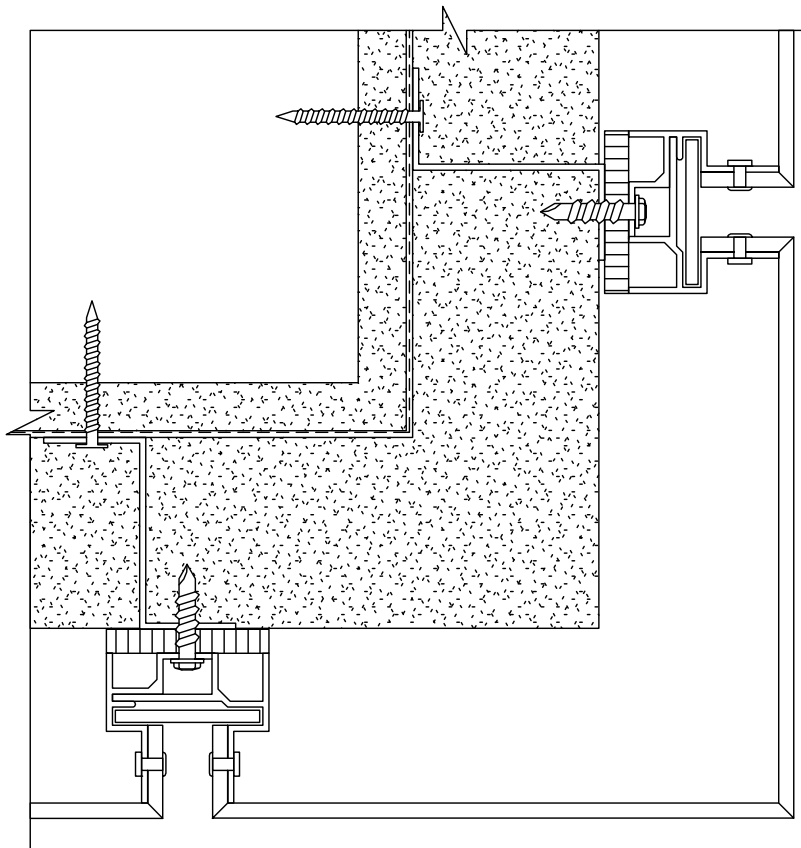
OUTSIDE CORNER DETAIL (TOP VIEW) S40
