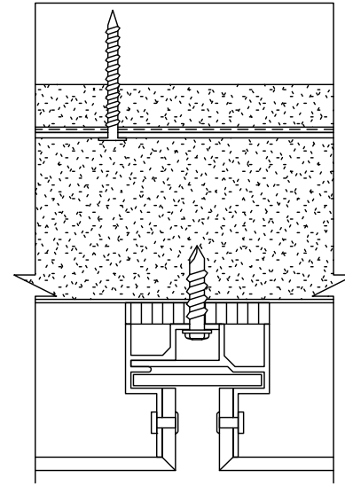
TYP. HORIZONTAL PANEL JOINT DETAIL
