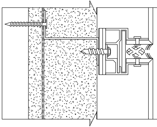
TYP. HORIZONTAL PANEL JOINT DETAIL
