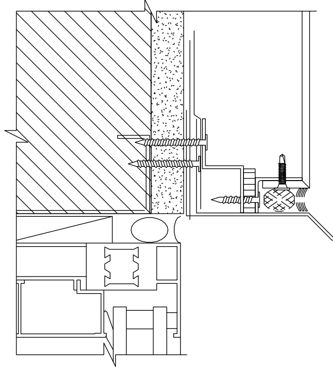
WINDOW / DOOR HEAD S10
